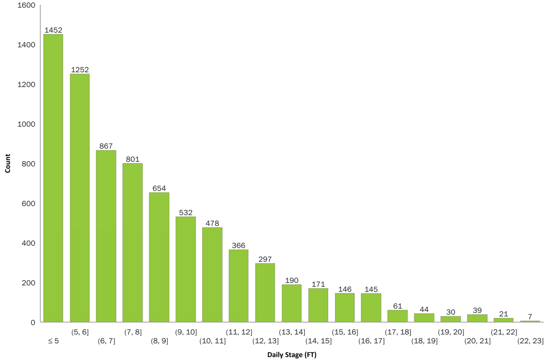
Histogram of Daily Stage for Mississippi River at Rock Island (Lock and Dam 15) from 2000 to 2020 Gage Zero Elevation = 542.50 FT
